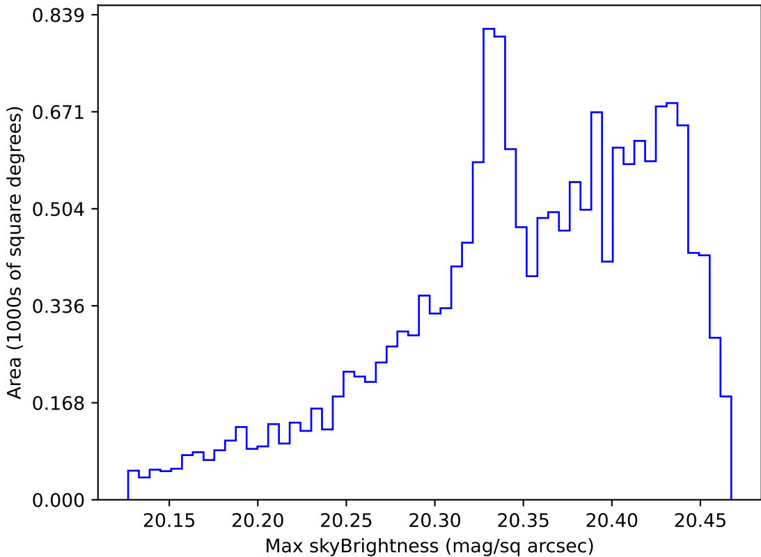
ddf_acor_sf25_lsf40_lsr10_v3.4_10yrs WFD i band: Max skyBrightness
