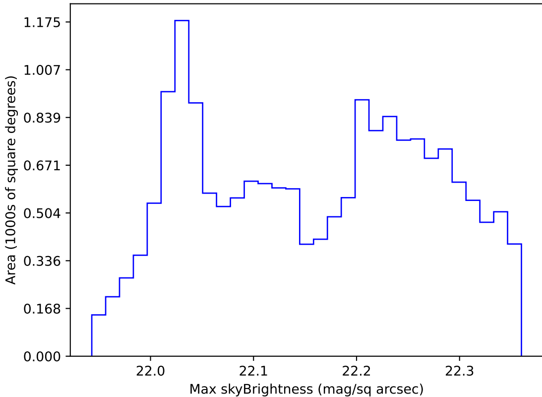
ddf_acor_sf25_lsf40_lsr10_v3.4_10yrs WFD g band: Max skyBrightness
