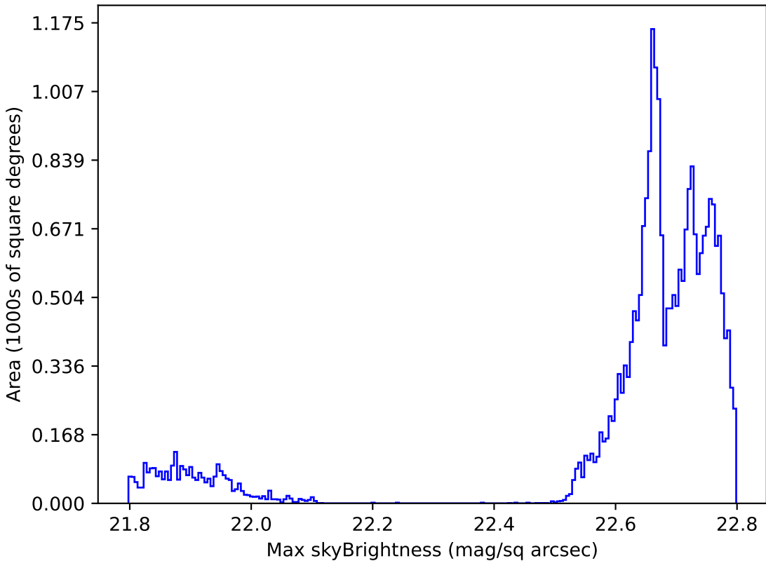
ddf_acor_sf25_lsf40_lsr10_v3.4_10yrs All sky all bands: Max skyBrightness
