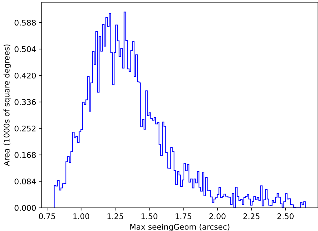
ddf_acor_sf25_lsf40_lsr10_v3.4_10yrs Yr 1 z band: Max seeingGeom
