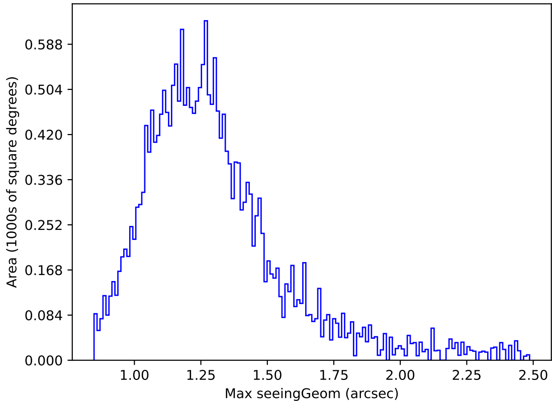
ddf_acor_sf25_lsf40_lsr10_v3.4_10yrs Yr 1 y band: Max seeingGeom
