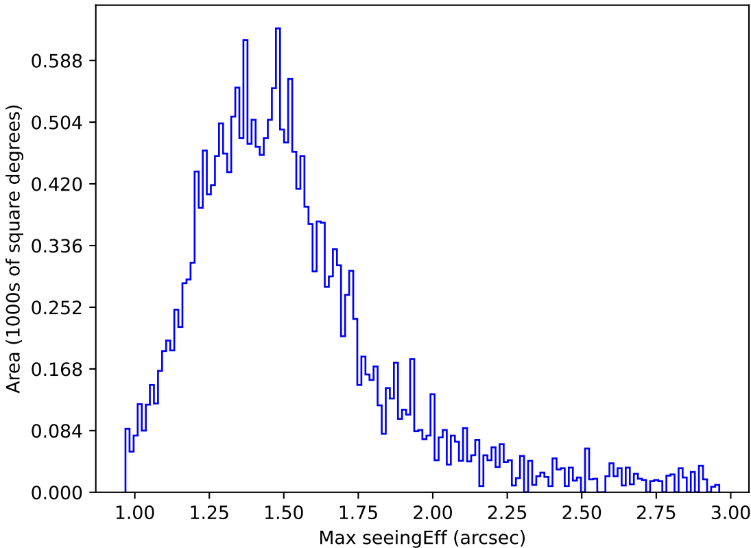
ddf_acor_sf25_lsf40_lsr10_v3.4_10yrs Yr 1 y band: Max seeingEff
