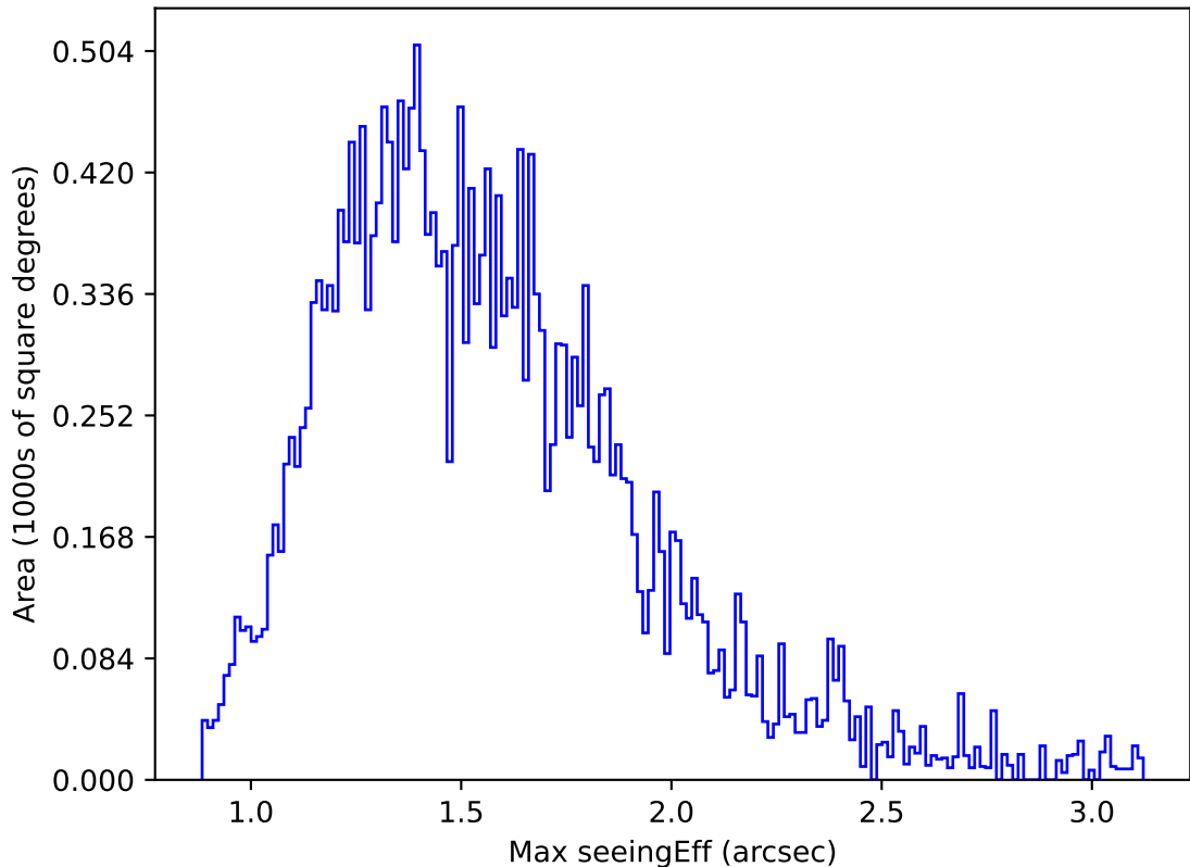
ddf_acor_sf25_lsf40_lsr10_v3.4_10yrs Yr 1 g band: Max seeingEff
