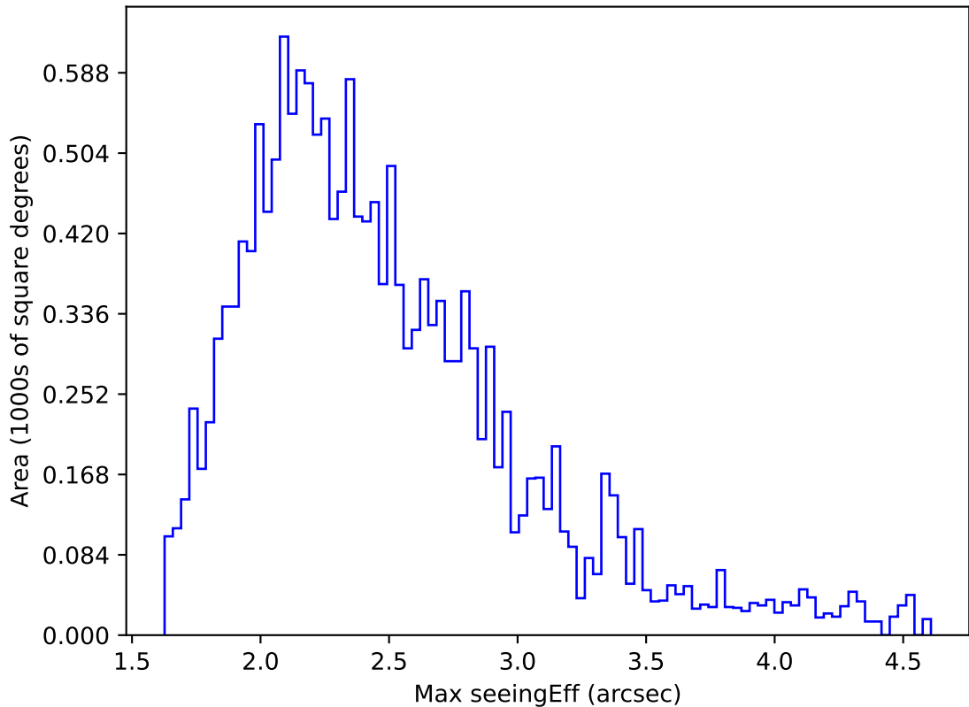
ddf_acor_sf25_lsf40_lsr10_v3.4_10yrs WFD y band: Max seeingEff
