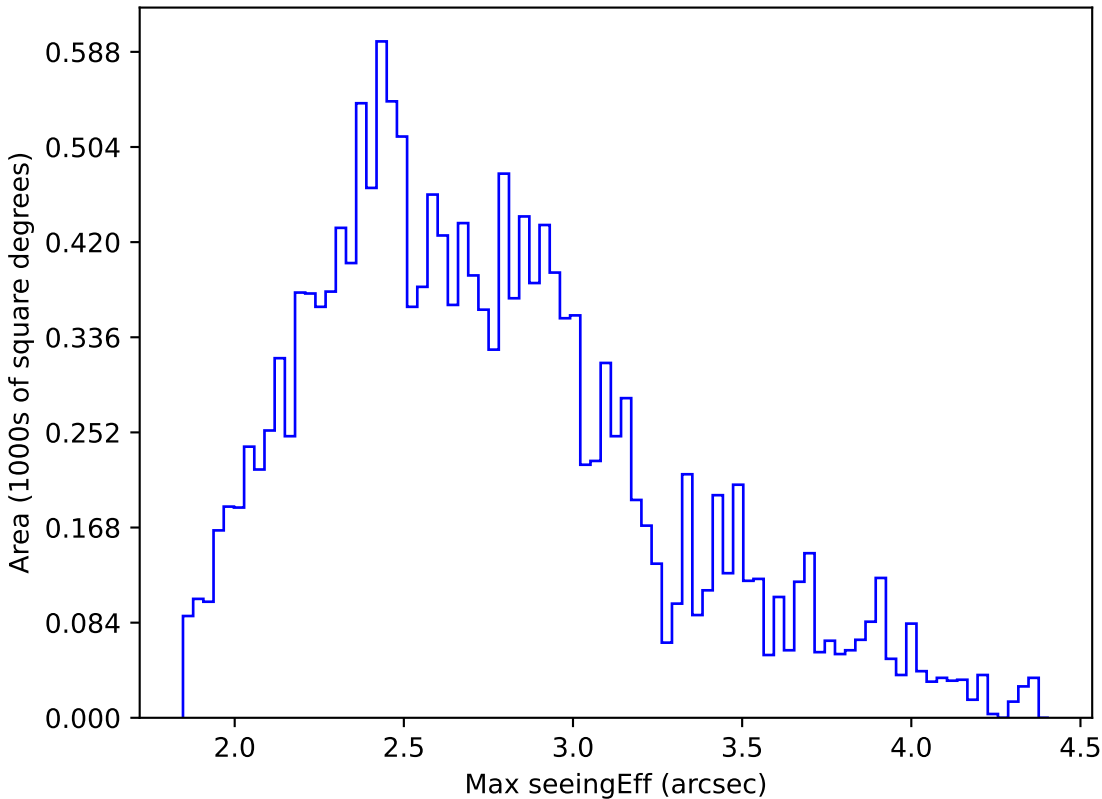
ddf_acor_sf25_lsf40_lsr10_v3.4_10yrs WFD r band: Max seeingEff
