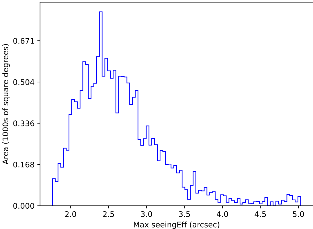
ddf_acor_sf25_lsf40_lsr10_v3.4_10yrs WFD i band: Max seeingEff
