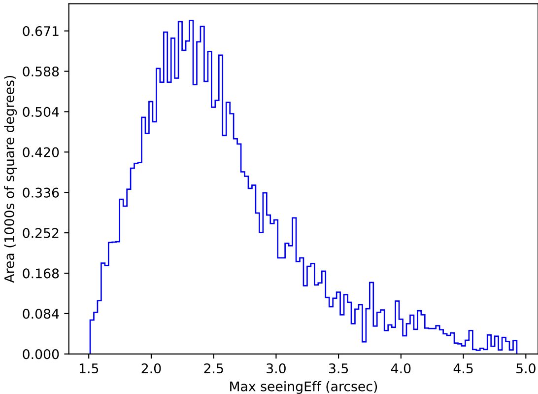
ddf_acor_sf25_lsf40_lsr10_v3.4_10yrs All sky z band: Max seeingEff
