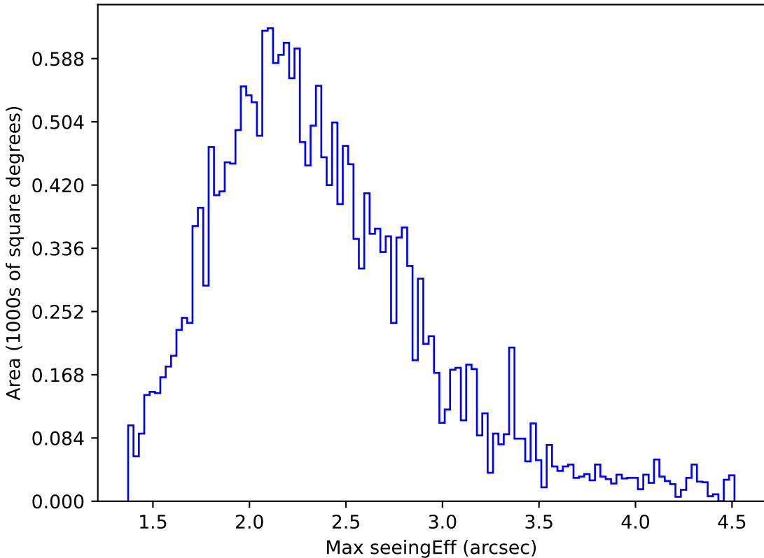
ddf_acor_sf25_ls40_lsr10_v3.4_10yrs All sky y band: Max seeingEff
