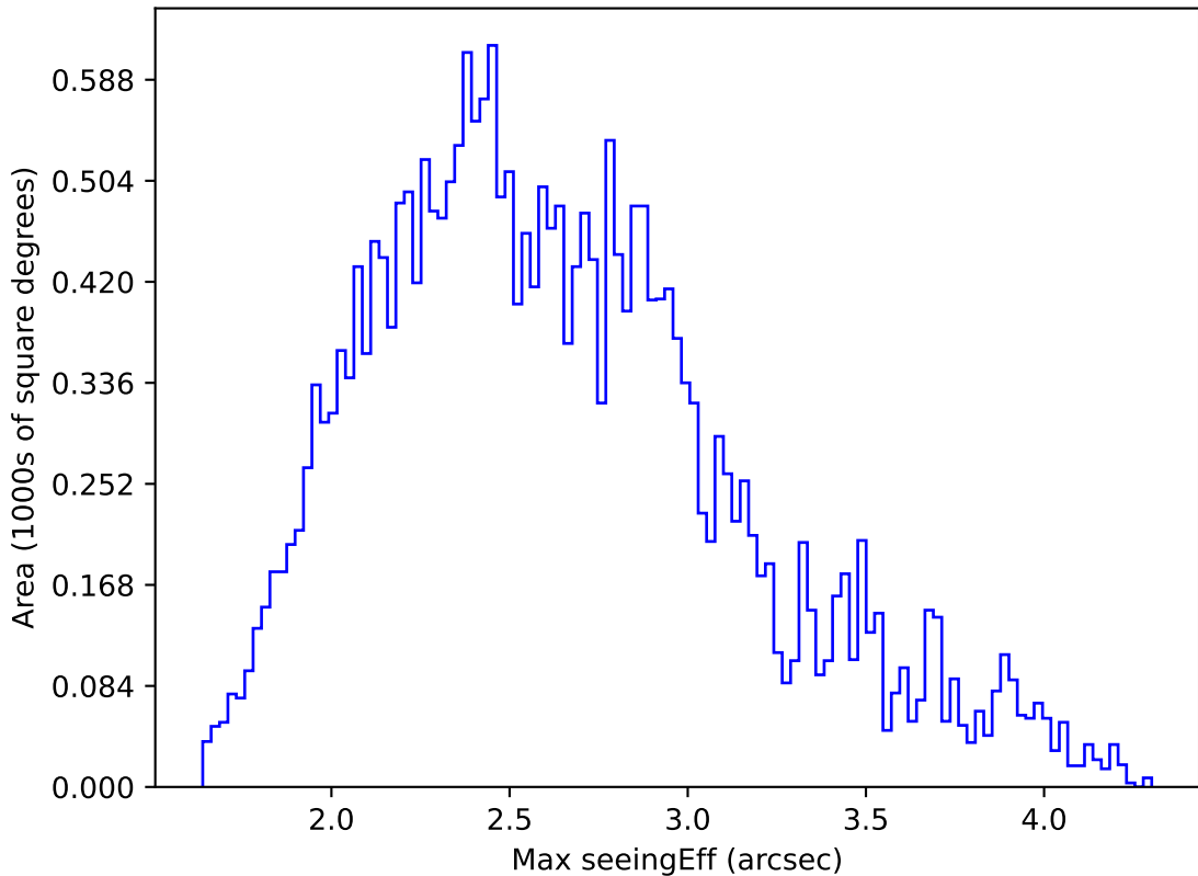
ddf_acor_sf25_lsf40_lsr10_v3.4_10yrs All sky r band: Max seeingEff
