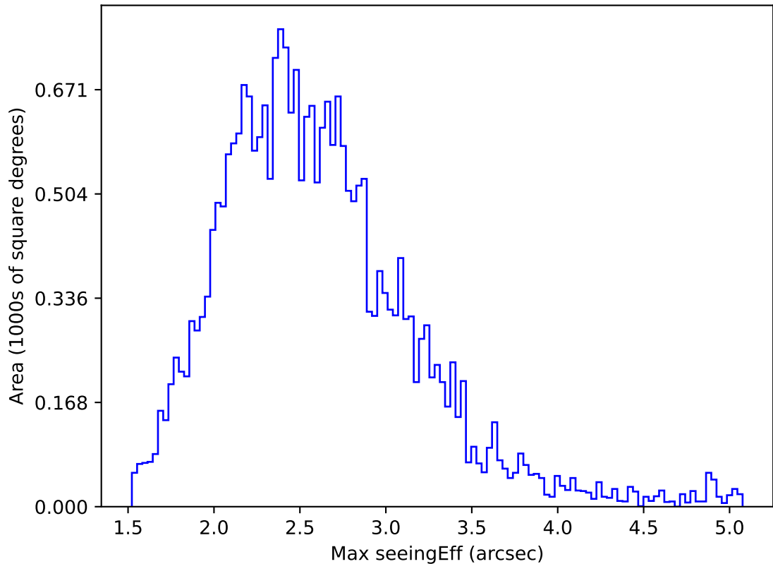
ddf_acor_sf25_lsf40_lsr10_v3.4_10yrs All sky i band: Max seeingEff
