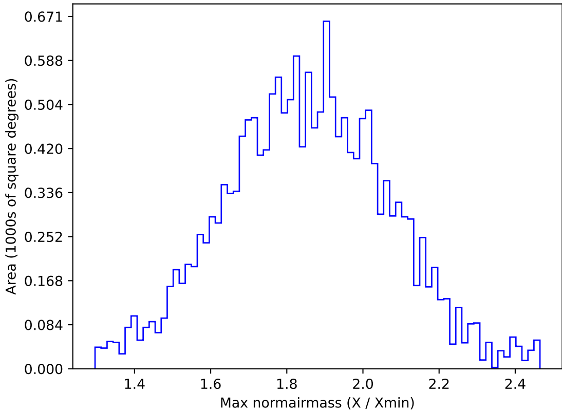
ddf_acor_sf25_lsf40_lsr10_v3.4_10yrs WFD g band: Max normairmass
