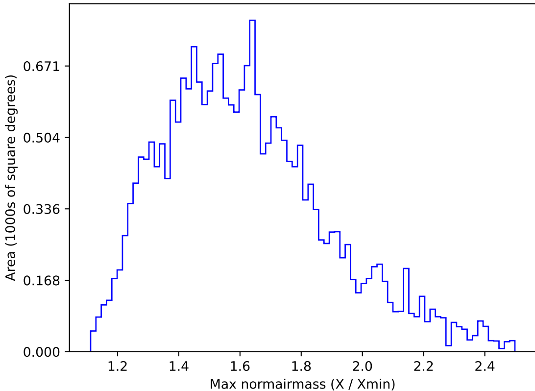
ddf_acor_sf25_lsf40_lsr10_v3.4_10yrs All sky u band: Max normairmass
