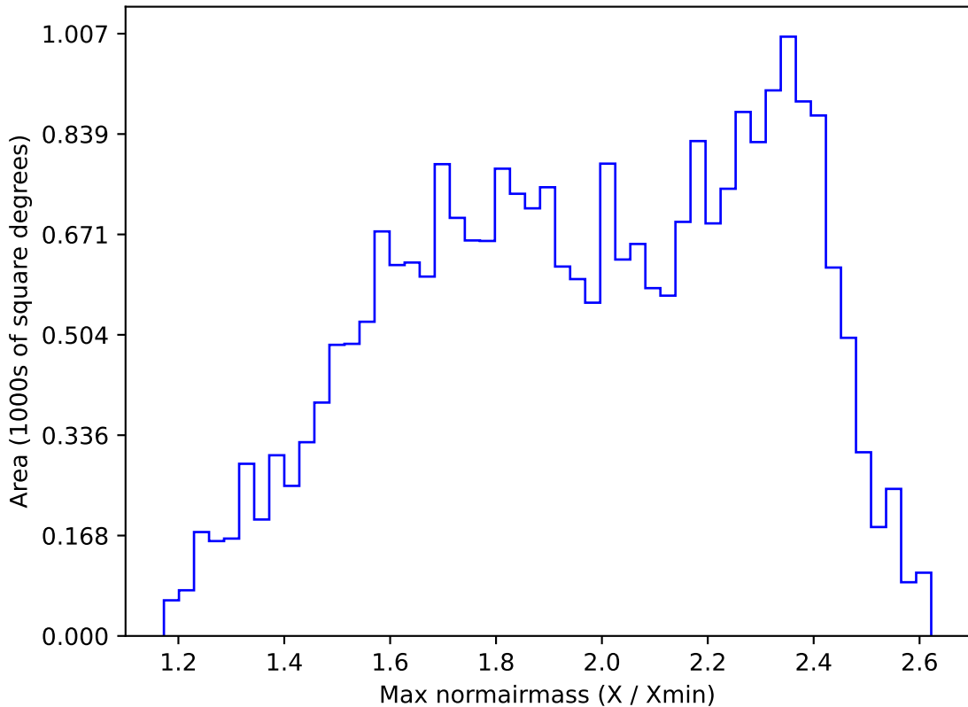
ddf_acor_sf25_lsf40_lsr10_v3.4_10yrs All sky r band: Max normairmass
