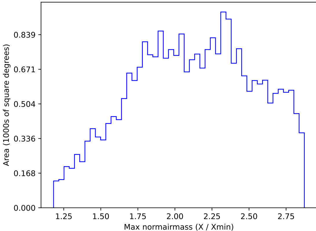
ddf_acor_sf25_lsf40_lsr10_v3.4_10yrs All sky i band: Max normairmass
