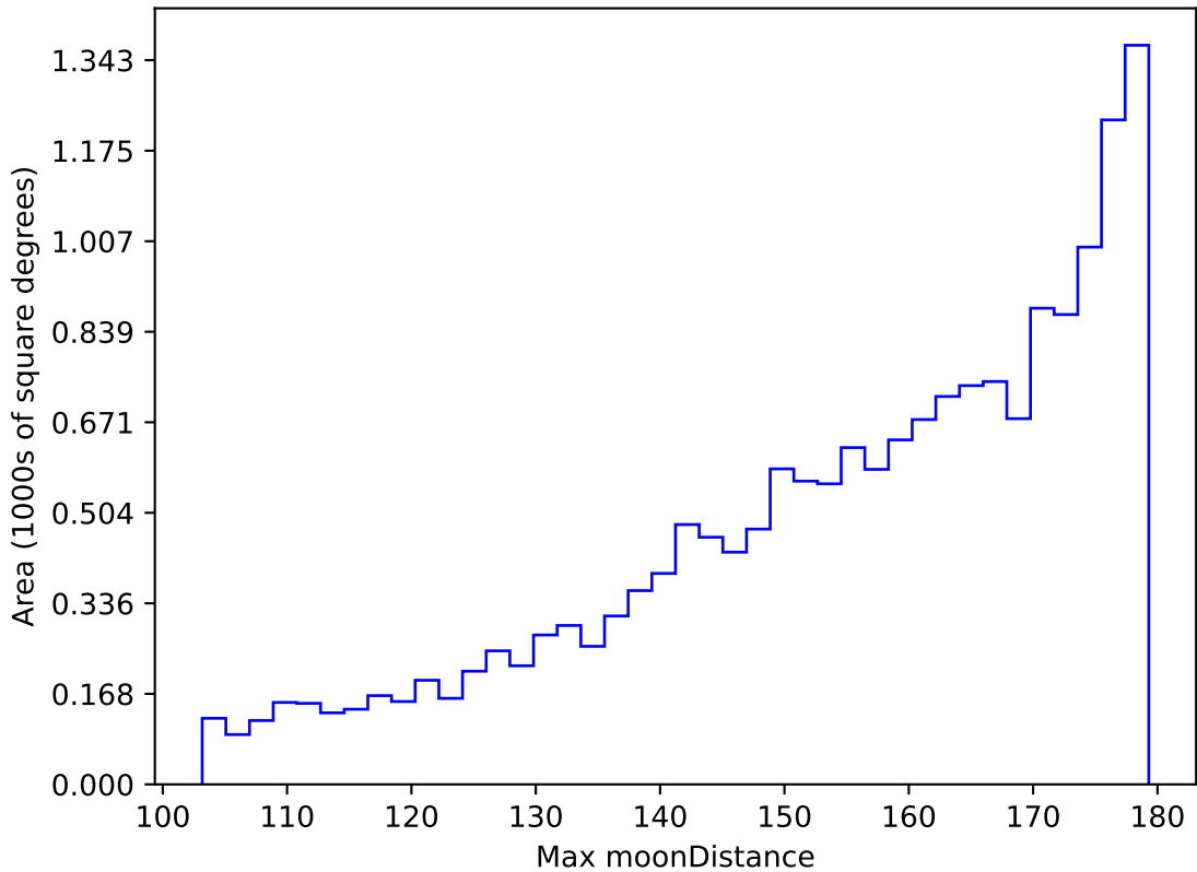
ddf_acor_sf25_lsf40_lsr10_v3.4_10yrs WFD i band: Max moonDistance
