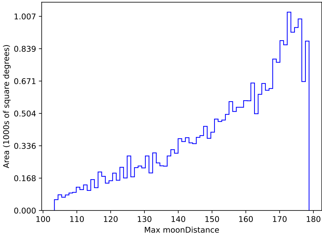
ddf_acor_sf25_lsf40_lsr10_v3.4_10yrs All sky g band: Max moonDistance
