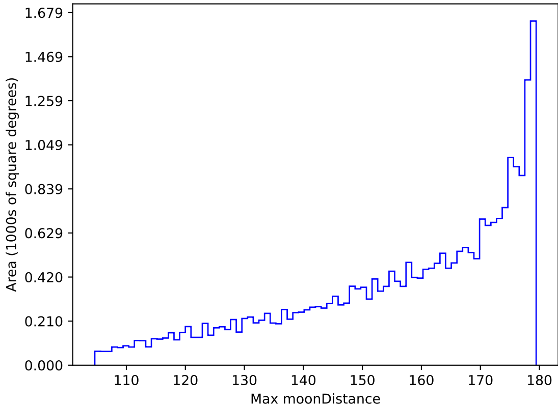
ddf_acor_sf25_lsf40_lsr10_v3.4_10yrs All sky all bands: Max moonDistance
