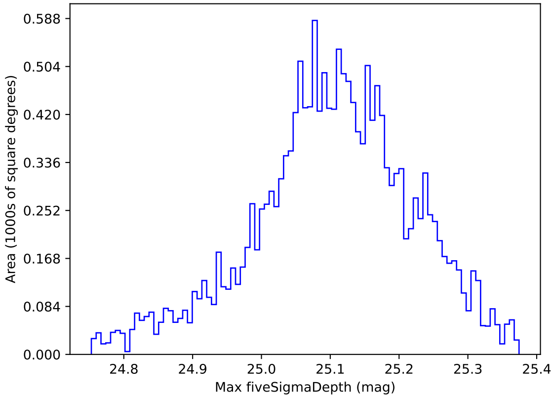
ddf_acor_sf25_lsf40_lsr10_v3.4_10yrs WFD all bands: Max fiveSigmaDepth
