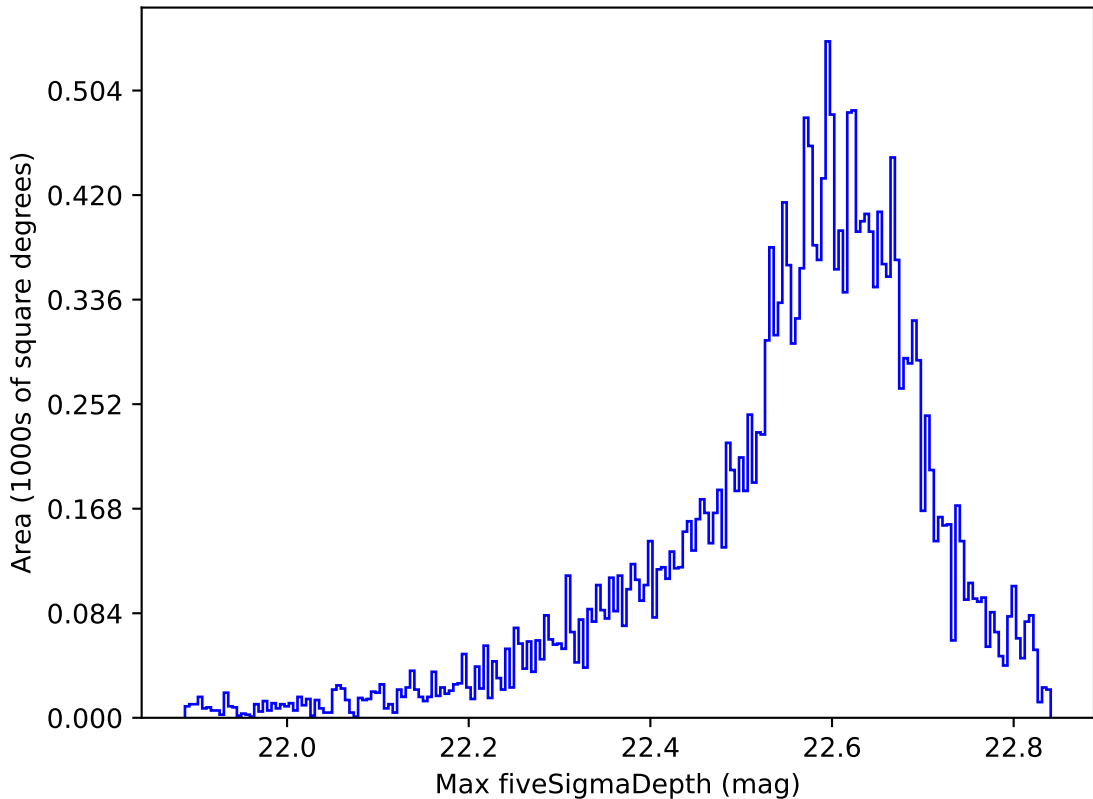
ddf_acor_sf25_lsf40_lsr10_v3.4_10yrs All sky y band: Max fiveSigmaDepth
