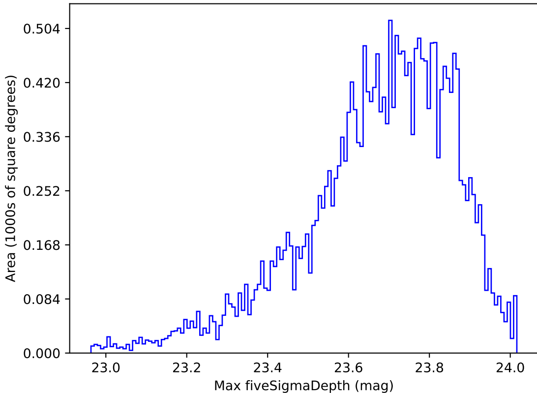
ddf_acor_sf25_lsf40_lsr10_v3.4_10yrs All sky u band: Max fiveSigmaDepth
