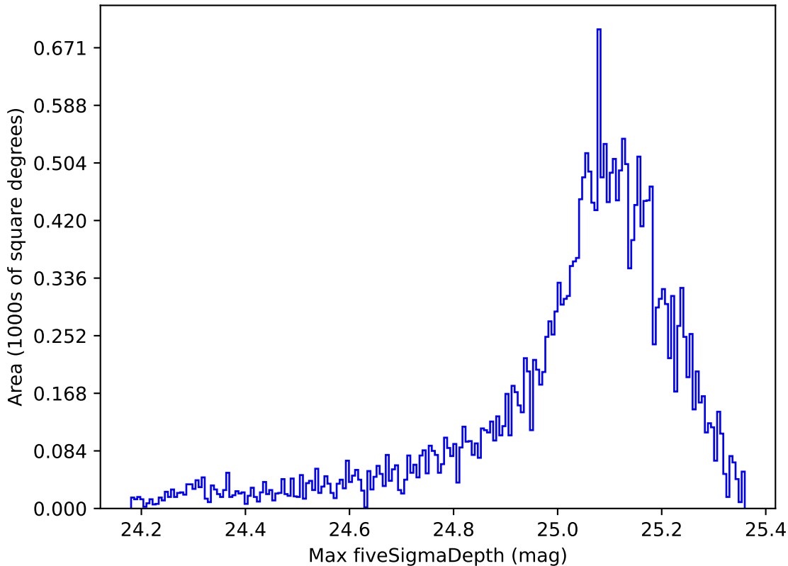
ddf_acor_sf25_lsf40_lsr10_v3.4_10yrs All sky g band: Max fiveSigmaDepth
