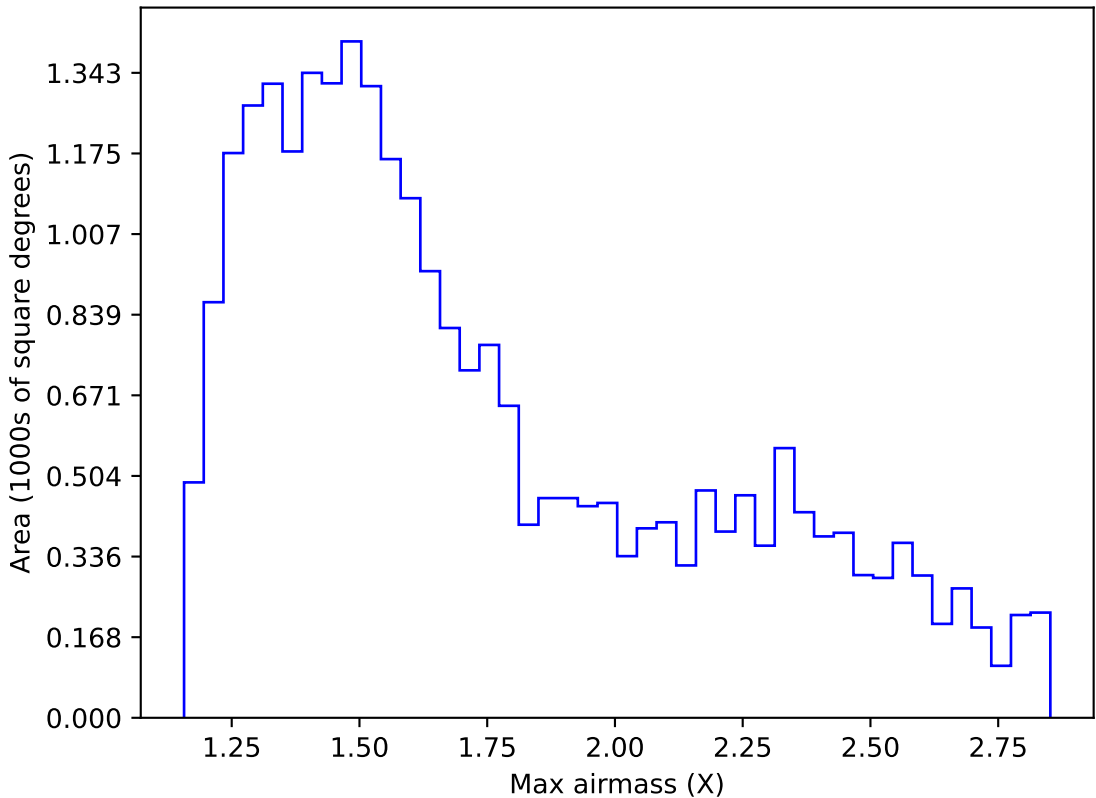
ddf_acor_sf25_lsf40_lsr10_v3.4_10yrs Yr 1 z band: Max airmass
