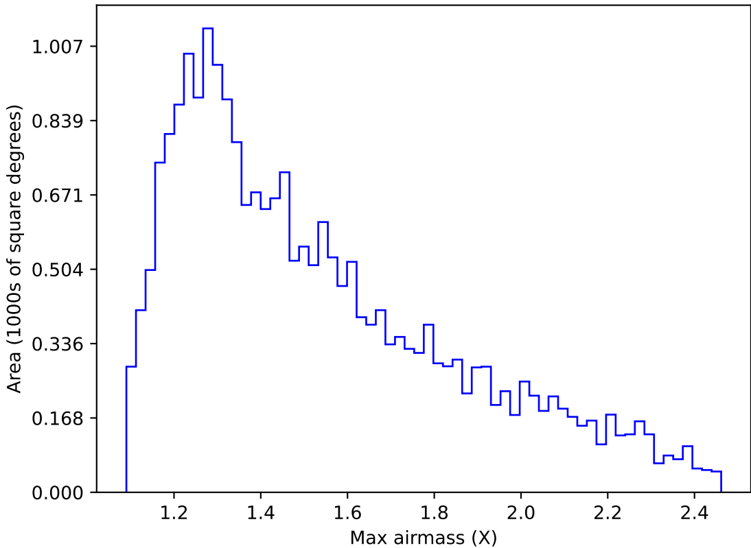
ddf_acor_sf25_lsf40_lsr10_v3.4_10yrs Yr 1 u band: Max airmass
