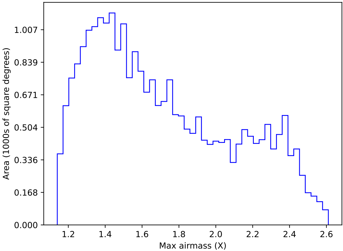
ddf_acor_sf25_lsf40_lsr10_v3.4_10yrs Yr 1 r band: Max airmass
