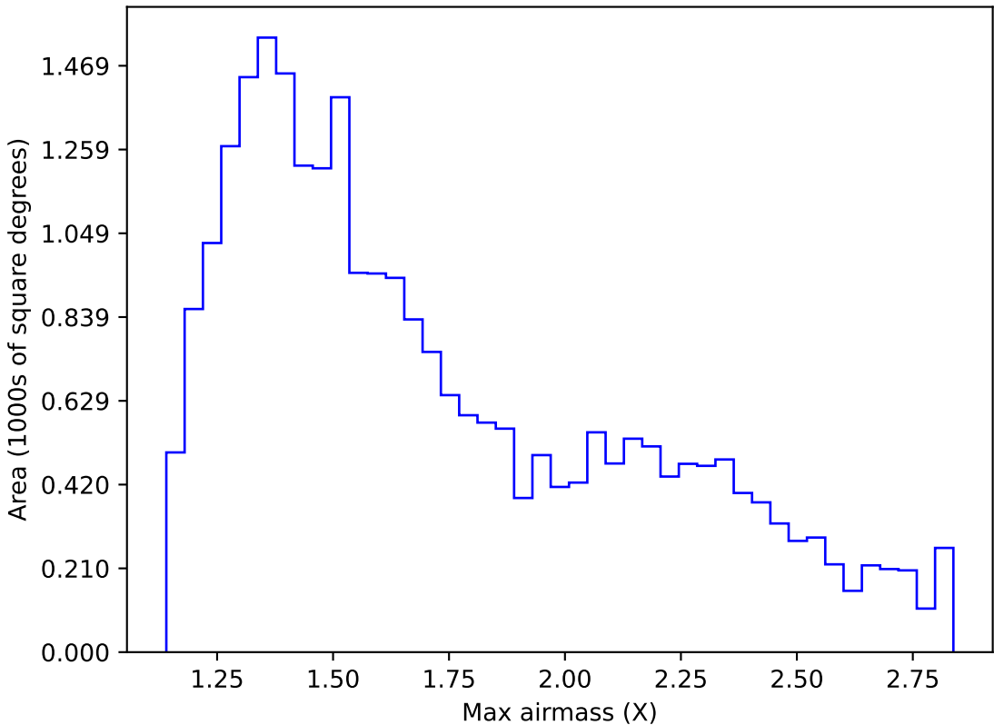
ddf_acor_sf25_lsf40_lsr10_v3.4_10yrs Yr 1 i band: Max airmass
