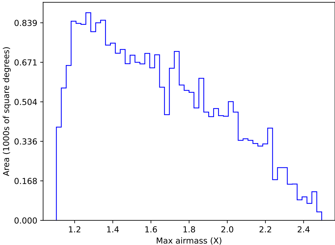
ddf_acor_sf25_lsf40_lsr10_v3.4_10yrs Yr 1 g band: Max airmass
