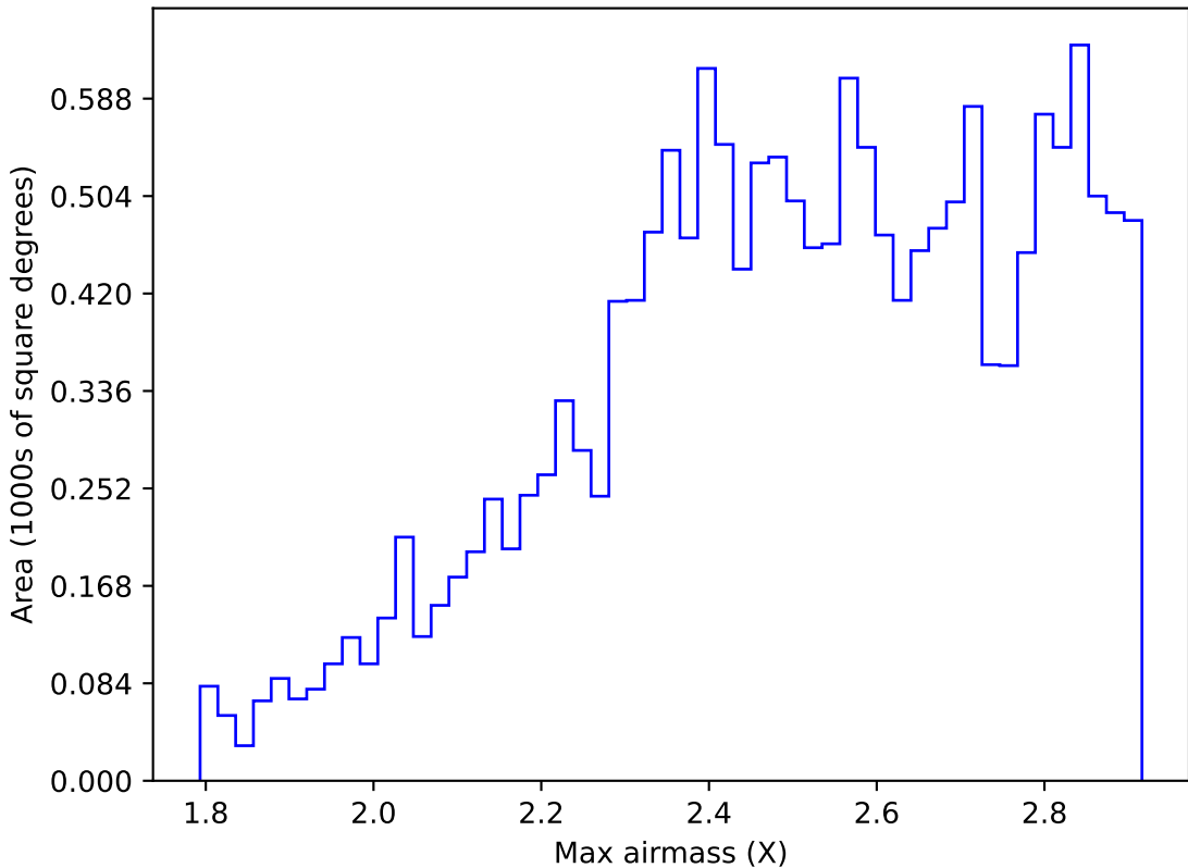
ddf_acor_sf25_lsf40_lsr10_v3.4_10yrs WFD z band: Max airmass
