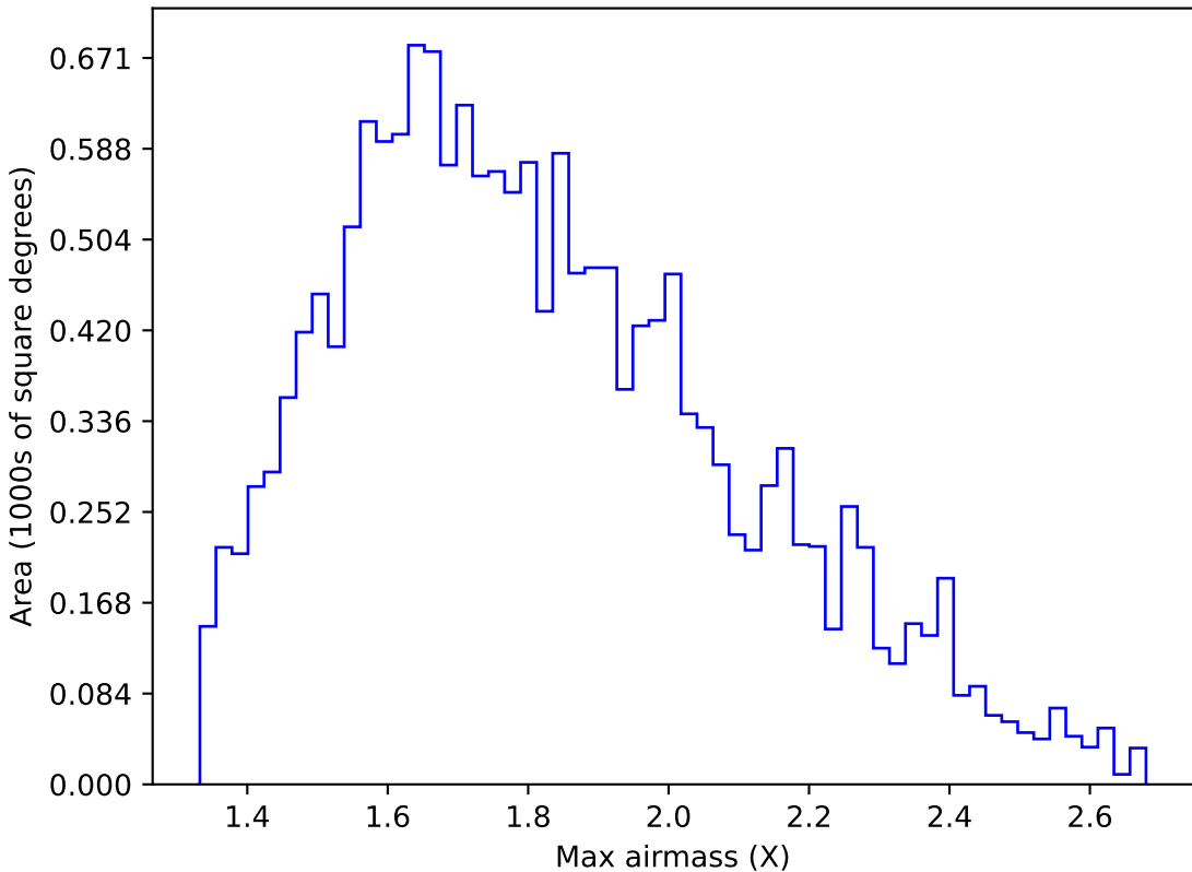
ddf_acor_sf25_lsf40_lsr10_v3.4_10yrs WFD u band: Max airmass
