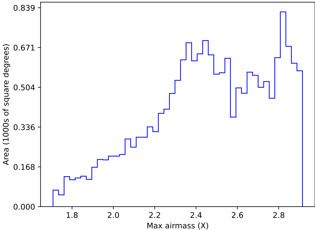
ddf_acor_sf25_lsf40_lsr10_v3.4_10yrs WFD i band: Max airmass
