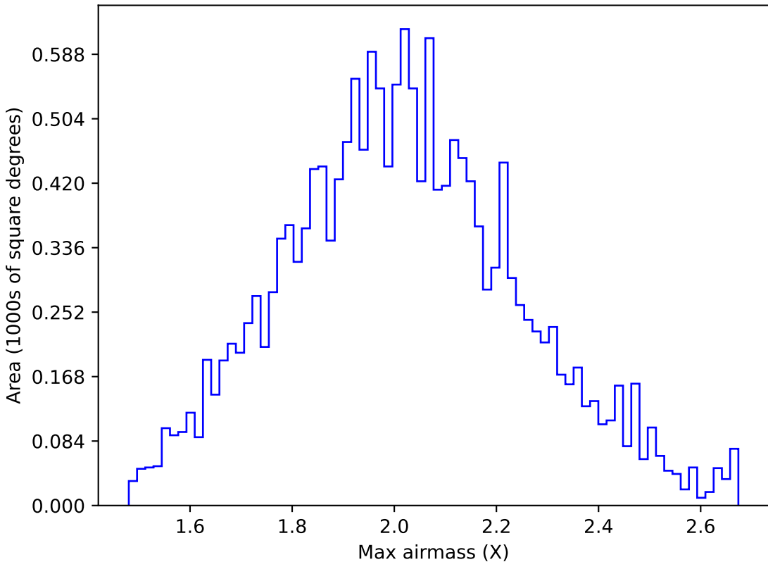
ddf_acor_sf25_lsf40_lsr10_v3.4_10yrs WFD g band: Max airmass
