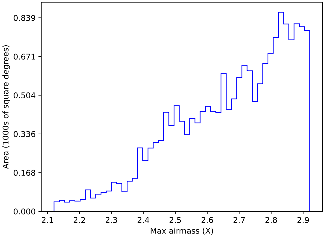
ddf_acor_sf25_lsf40_lsr10_v3.4_10yrs WFD all bands: Max airmass
