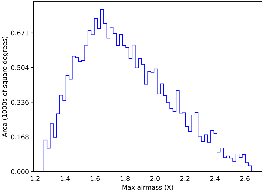
ddf_acor_sf25_lsf40_lsr10_v3.4_10yrs All sky u band: Max airmass
