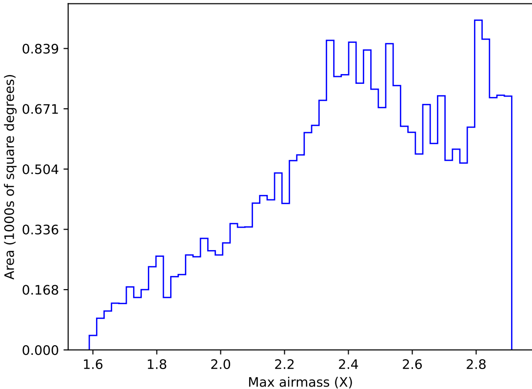
ddf_acor_sf25_lsf40_lsr10_v3.4_10yrs All sky i band: Max airmass
