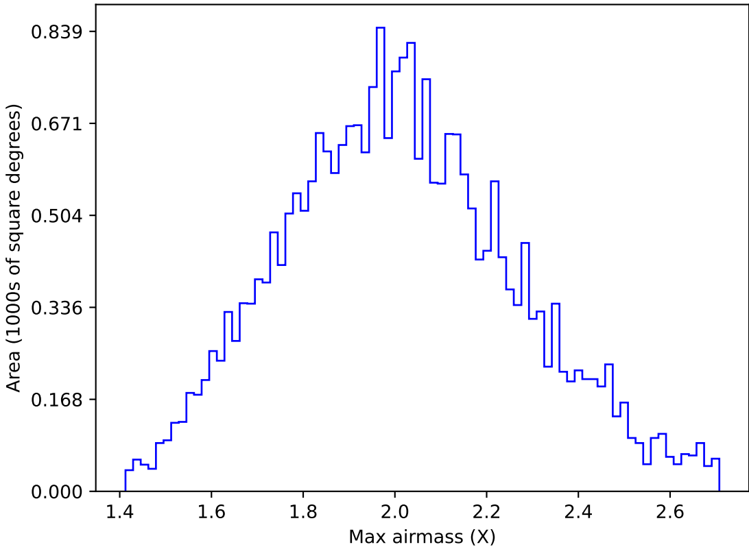
ddf_acor_sf25_lsf40_lsr10_v3.4_10yrs All sky g band: Max airmass
