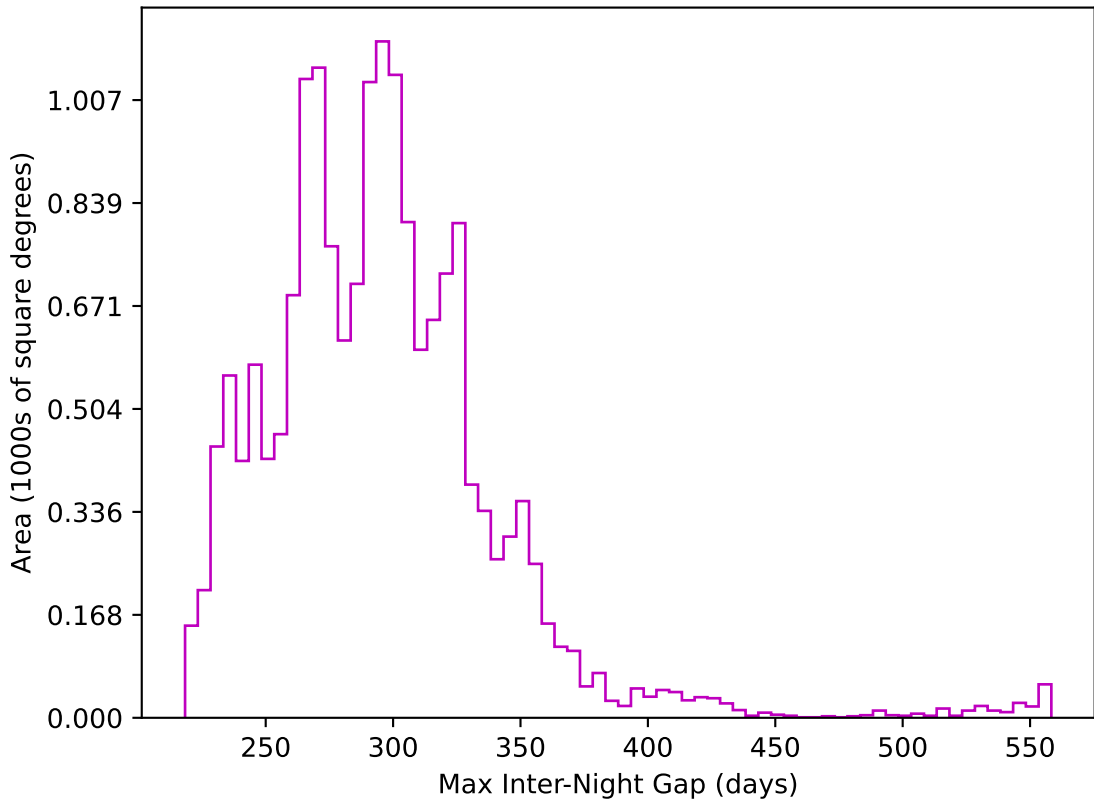
ddf_acor_sf25_lsf40_lsr10_v3.4_10yrs WFD z band: Max Inter-Night Gap
