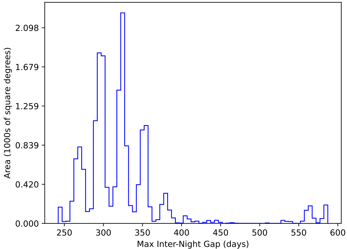
ddf_acor_sf25_lsf40_lsr10_v3.4_10yrs WFD y band: Max Inter-Night Gap
