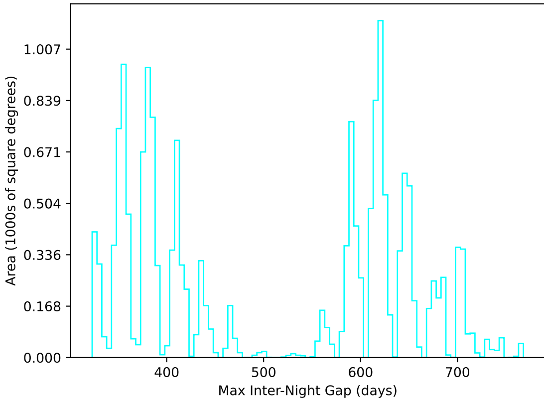
ddf_acor_sf25_lsf40_lsr10_v3.4_10yrs WFD u band: Max Inter-Night Gap
