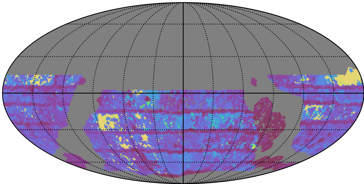
ddf_acor_sf25_lsf40_lsr10_v3.4_10yrs WFD r band: Max Inter-Night Gap
