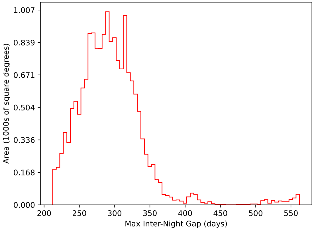
ddf_acor_sf25_lsf40_lsr10_v3.4_10yrs WFD i band: Max Inter-Night Gap
