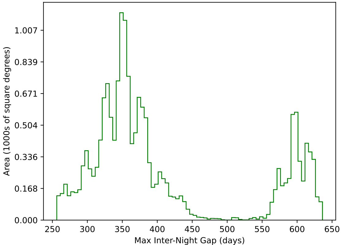
ddf_acor_sf25_lsf40_lsr10_v3.4_10yrs WFD g band: Max Inter-Night Gap
