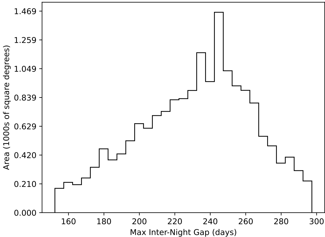
ddf_acor_sf25_lsf40_lsr10_v3.4_10yrs WFD all bands: Max Inter-Night Gap
