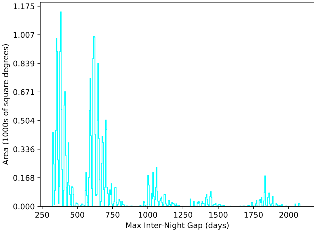
ddf_acor_sf25_lsf40_lsr10_v3.4_10yrs All sky u band: Max Inter-Night Gap
