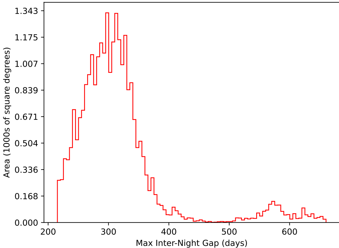
ddf_acor_sf25_lsf40_lsr10_v3.4_10yrs All sky i band: Max Inter-Night Gap
