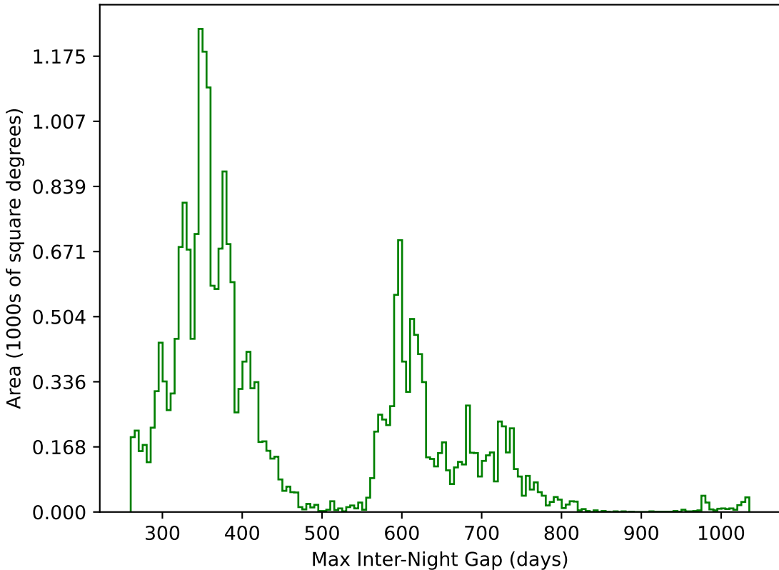
ddf_acor_sf25_lsf40_lsr10_v3.4_10yrs All sky g band: Max Inter-Night Gap
