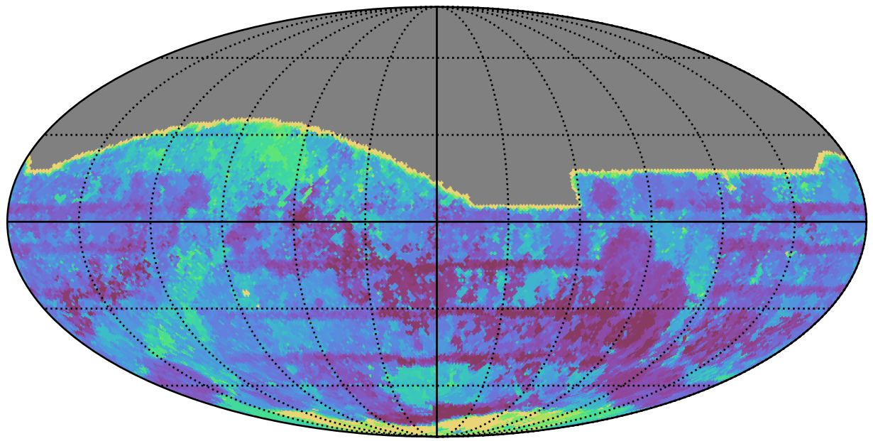
ddf_acor_sf25_lsf40_lsr10_v3.4_10yrs All sky all bands: Max Inter-Night Gap
