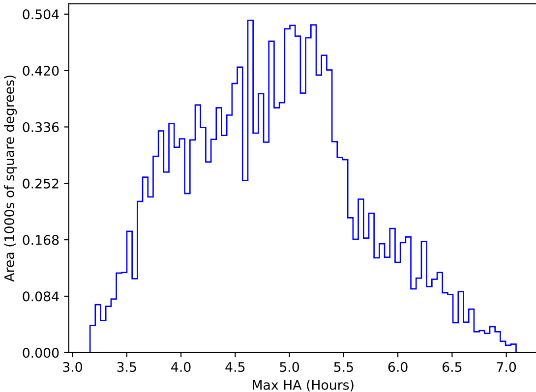
ddf_acor_sf25_lsf40_lsr10_v3.4_10yrs WFD i band: Max HA
